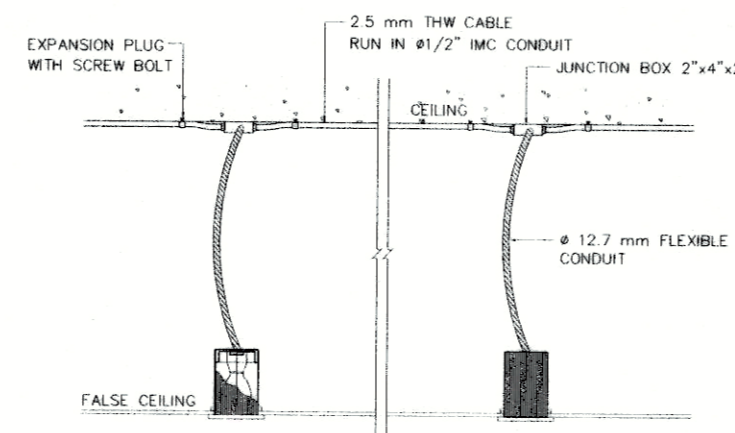
INSTALLATION DETAIL OF RECESSED DOWNLIGHT LUMINAIRE
