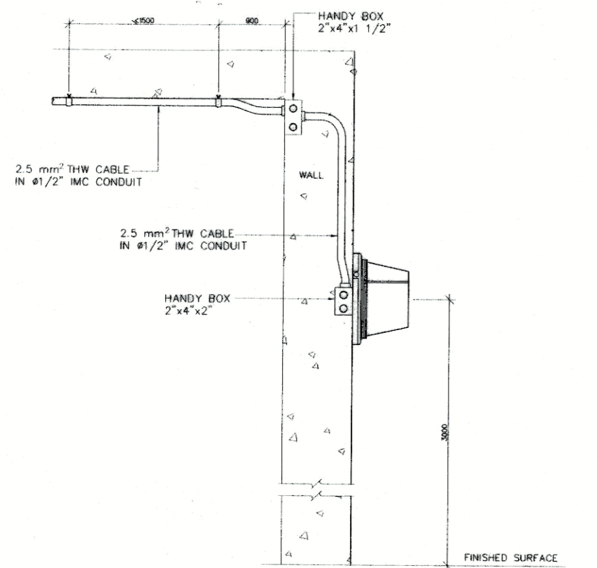
INSTALLATION DETAIL OF EXTERIOR BUILDING LUMINAIRE
