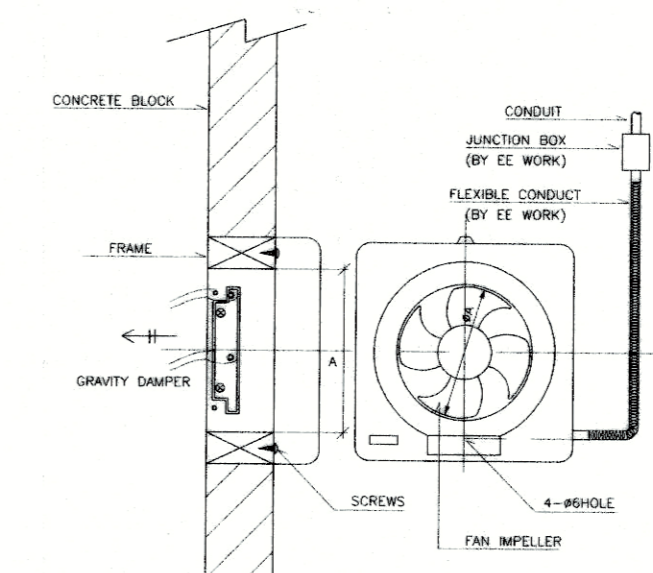
PROPELLER FAN (WALL MOUNTED TYPE)
