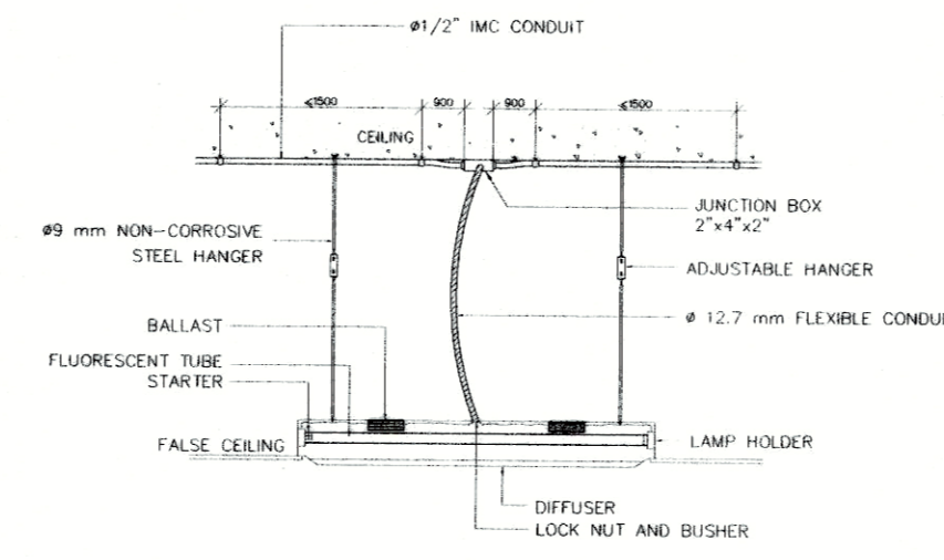
INSTALLATION DETAIL OF RECESSED FLUORESCENT LUMINAIRE ON FIXED CEILING
