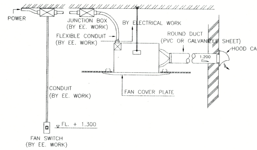
CEILING FAN TYPICAL DETAIL
