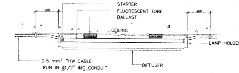
INSTALLATION DETAIL OF SURFACED FLUORESCENT LUMINAIRE
